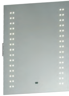
PERLE SHAVER IR MIRROR IP44 13760 Mirrored glass & silver paint H: 600mm W: 500mm Proj: 50mm Int. LED 320 lumens
